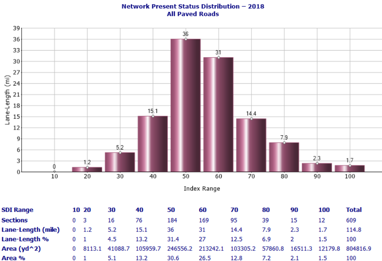
Figure 4.2: SDI Distribution; All Paved Roads
