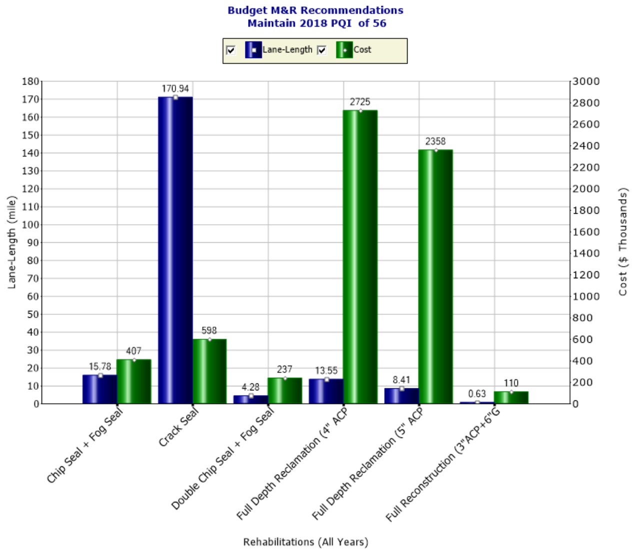
Figure 4.10: “Maintain 2018 PQI of 56” Recommended Rehabilitations by Treatment
