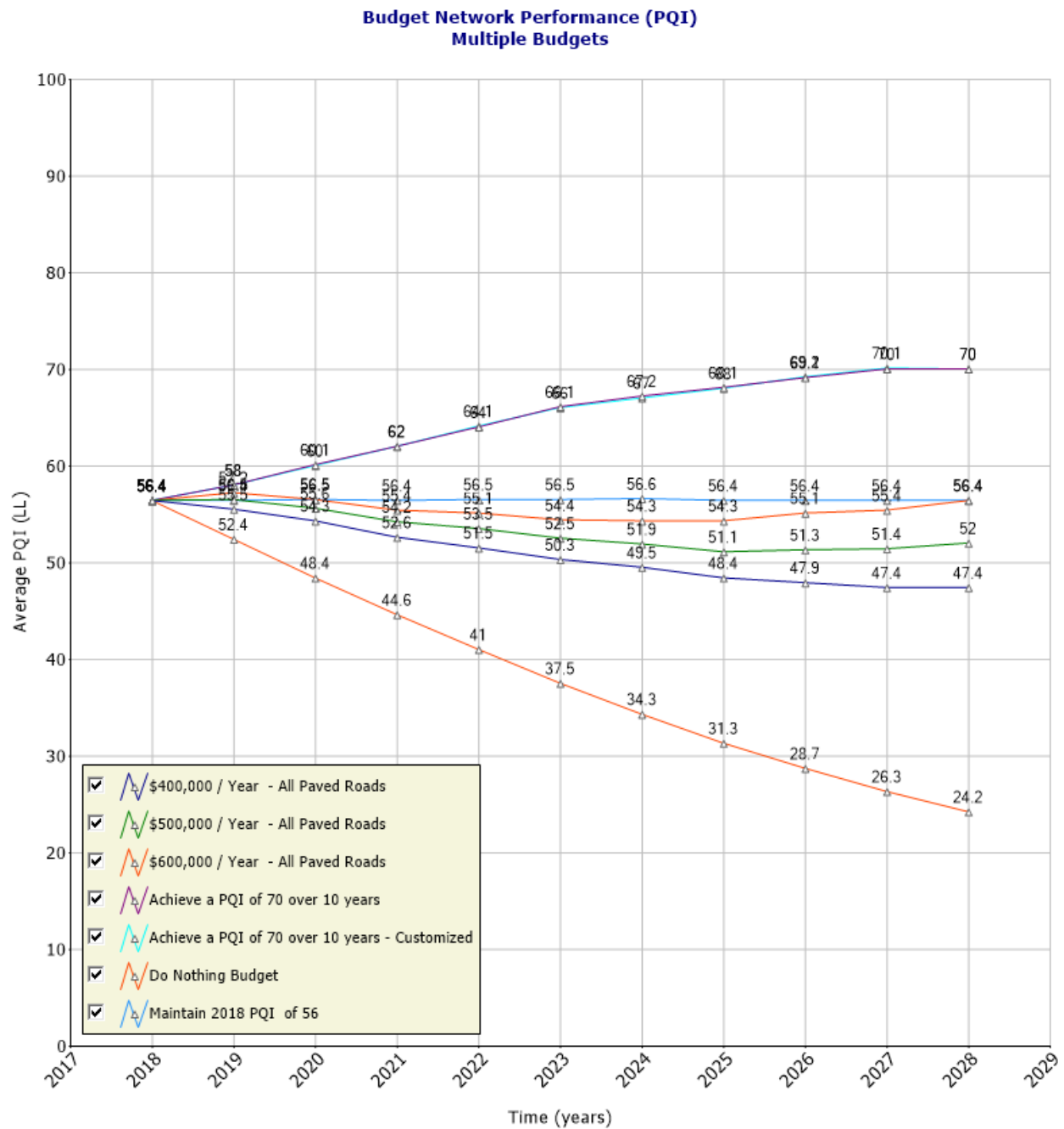
Figure 4.5: Funding Impact on Network Predicted Average PQI
