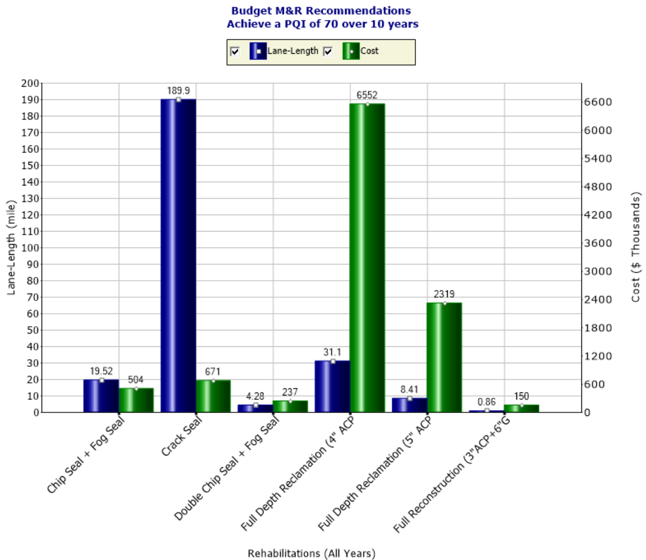
Figure 4.11: “Achieve a PQI of 70 over 10 years” Recommended Rehabilitations by Treatment
