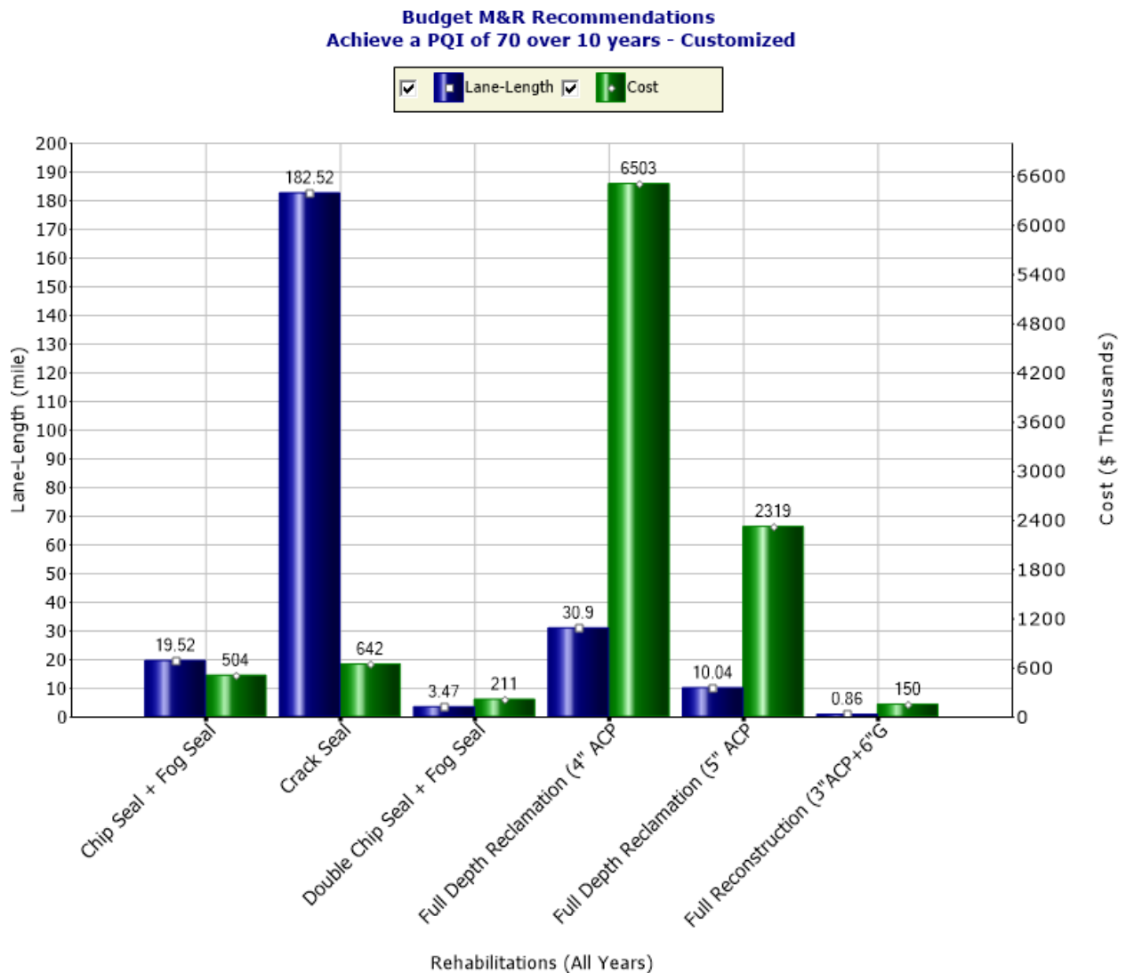
Figure 4.12: “Achieve a PQI of 70 over 10 years - Customized” Recommended Rehabilitations by Treatment
