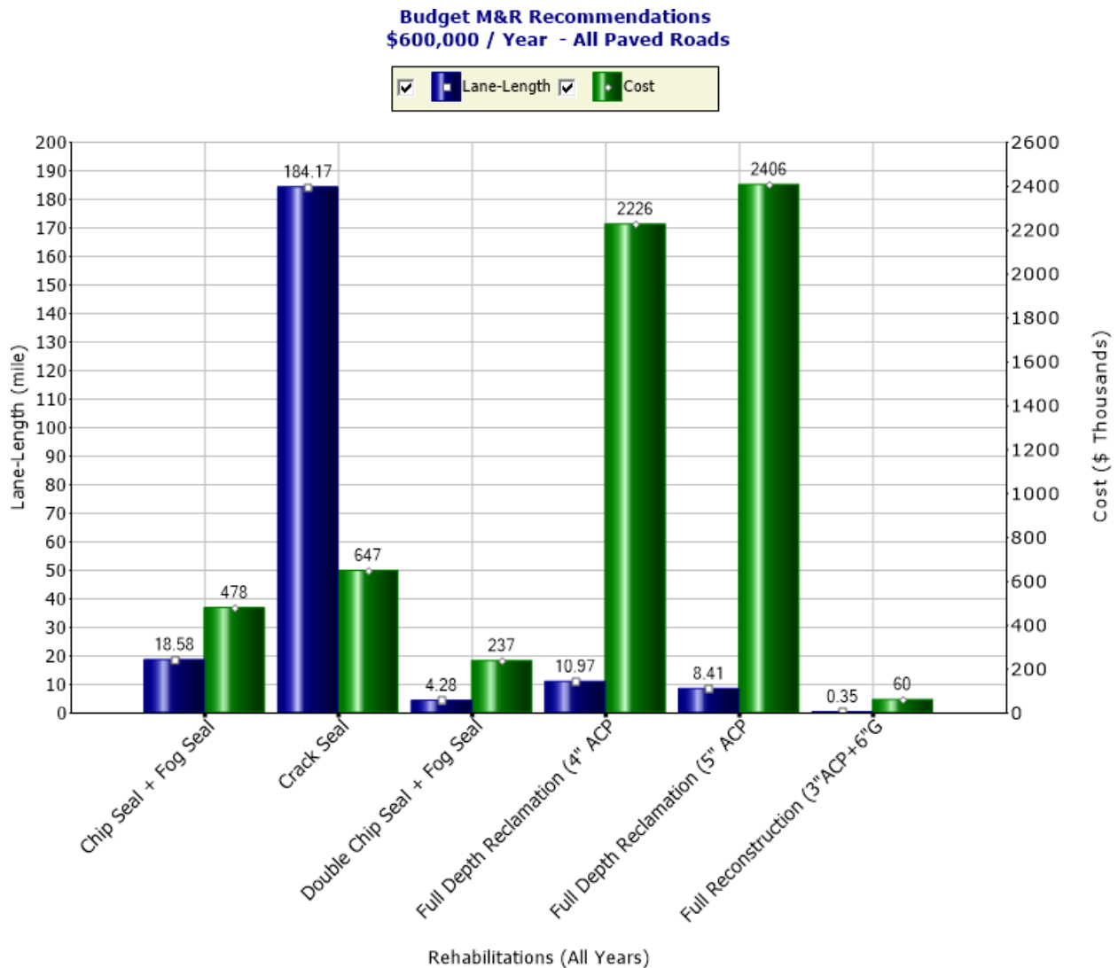
Figure 4.9: $600,000/Year Recommended Rehabilitations by Treatment
