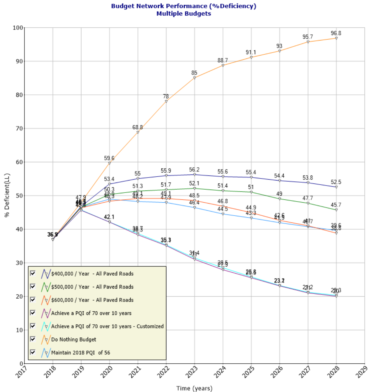
Figure 4.6: Funding Impact on Network Predicted Average Deficiency
