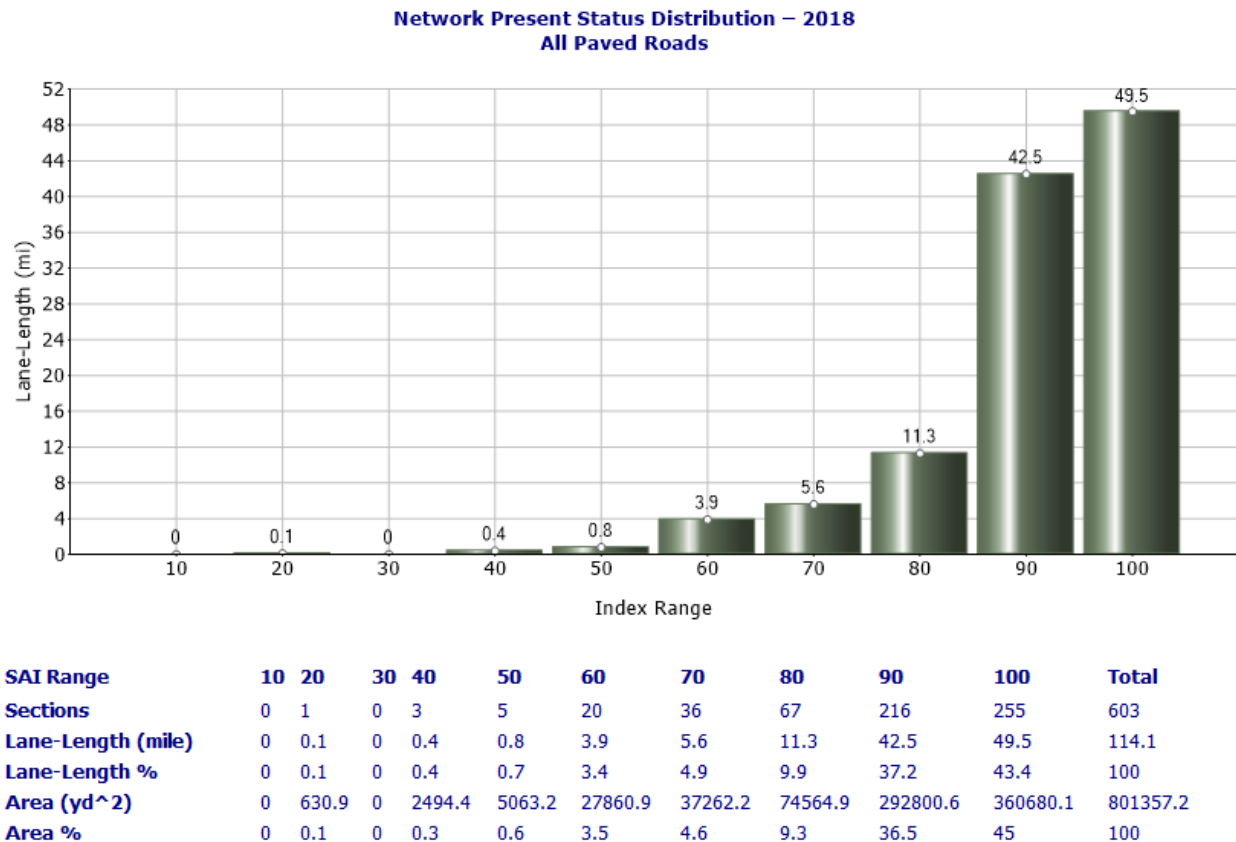
Figure 4.3: SAI Distribution; All Paved Roads
