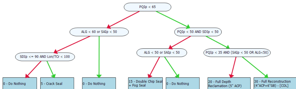
Figure 3.2: Flexible Pavement – Collector Roads Decision Tree
