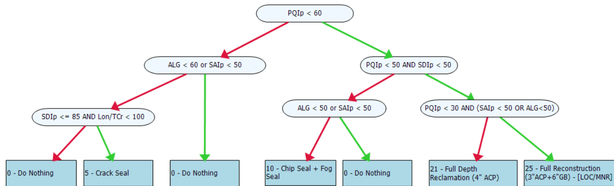
Figure 3.3: Flexible Pavement – Local/Minor Roads Decision Tree
