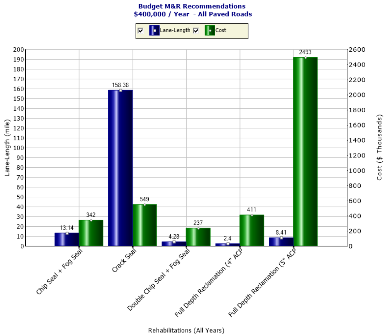
Figure 4.7: $400,000/Year Recommended Rehabilitations by Treatment
